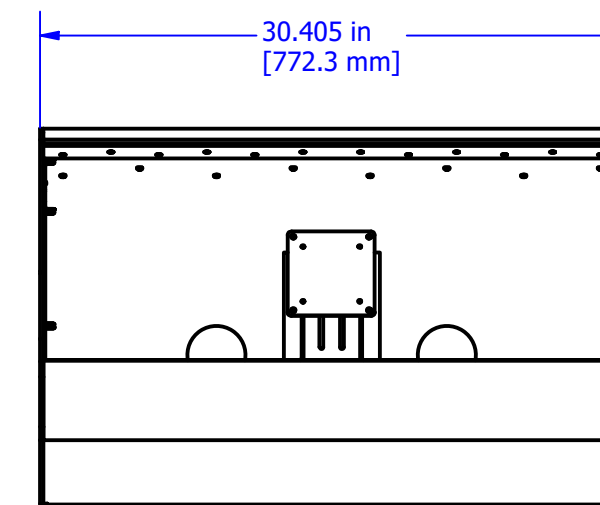
30 in DAW BUCKET, 921-0529 FOR AVID S3 or 921-0528 FOR WORK SURFACE CAN BE ADDED TO THE END OF ANY FRAME or IN THE 32 CHANNEL FRAME AS SHOWN IN 921-0536
