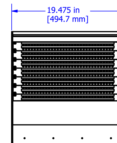
921-0527 19 in RACK SPACE BUCKET WITH 8U OF SPACE FOR PATCH BAY CAN BE ADDED TO THE END OF ANY FRAME
