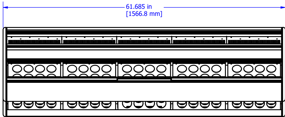
921-0535 32-CHANNEL SINGLE FRAME, 1-16, MASTER, 17-32
