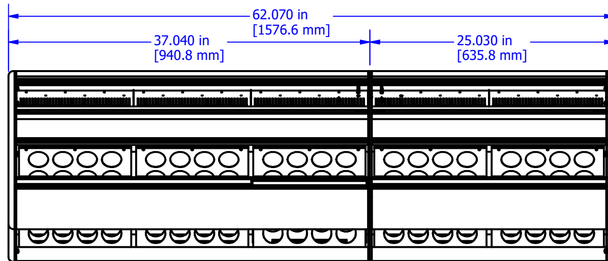
921-0537 32-CHANNEL SPLIT FRAME, 1-16, MASTER, 17-32
