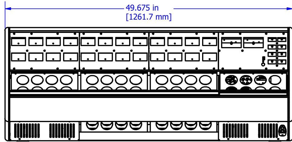
921-0534 STANDARD 24-CHANNEL FRAME
