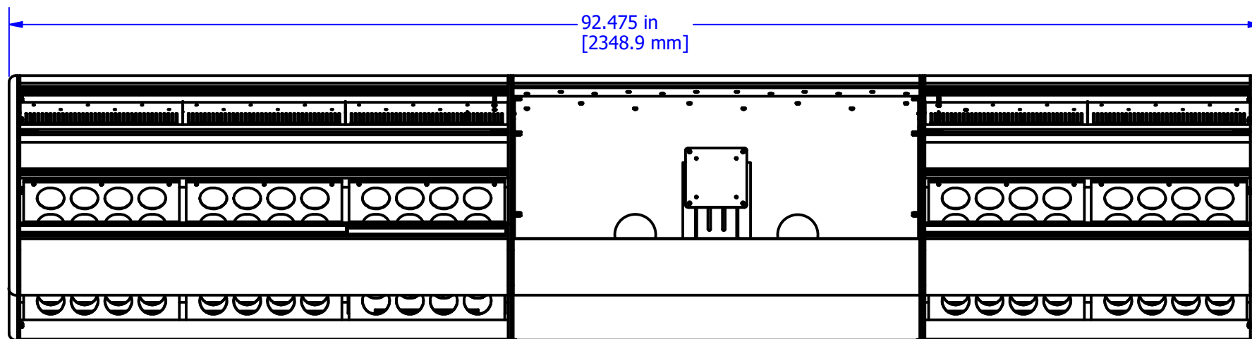
921-0536 32-CHANNEL w/ 30" DAW BUCKET FRAME ORDER CAN BE 1-16, MASTER, DAW, 17-32 or 1-16, DAW, MASTER, 17-32
